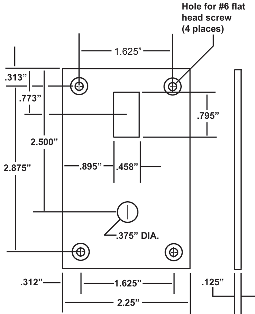
Dimensions of the (SHW) TCV Turns Counter
